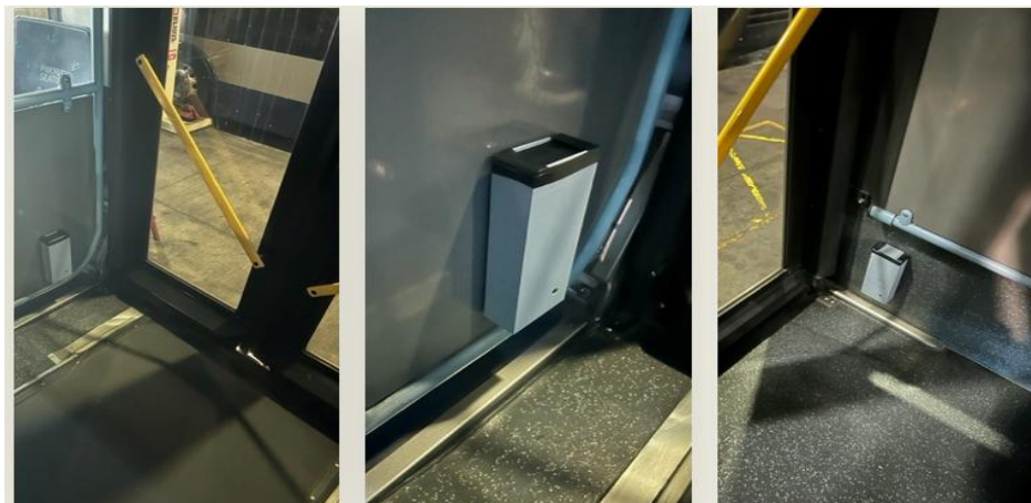
Figure 8 – O2O Recording Device and Positioning on Vehicle
